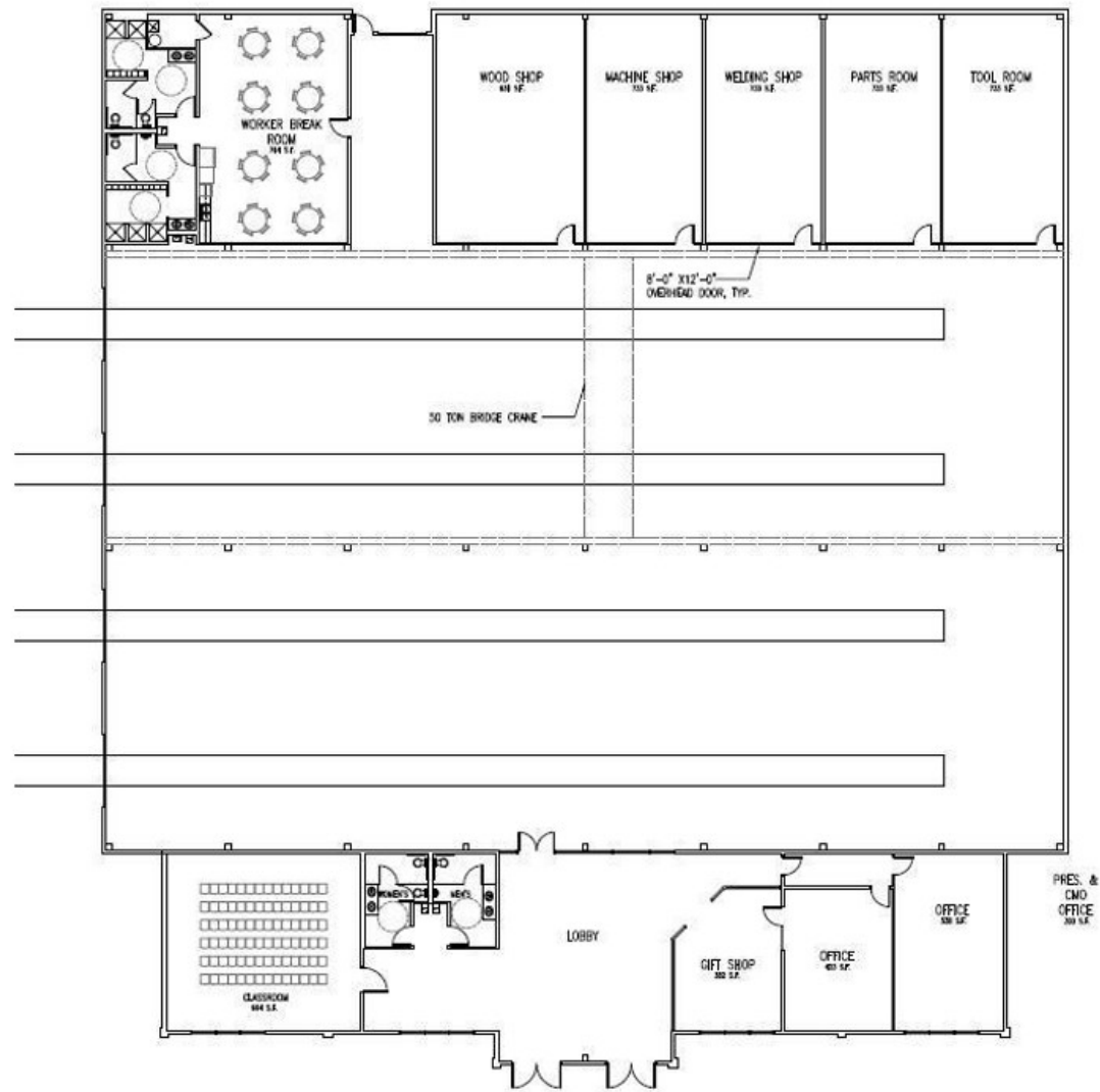
Floor Plan
