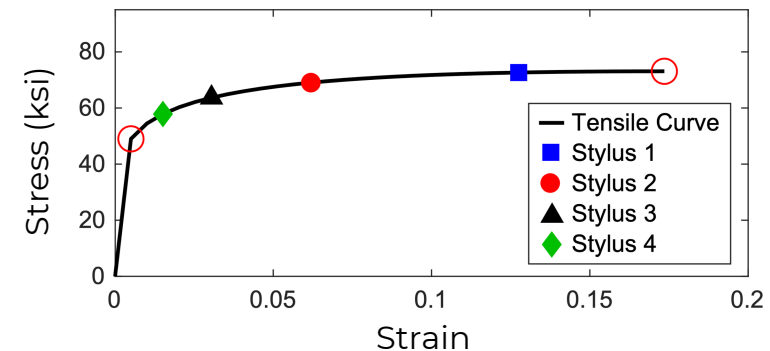
HSD Test Surface Strength Predictions
