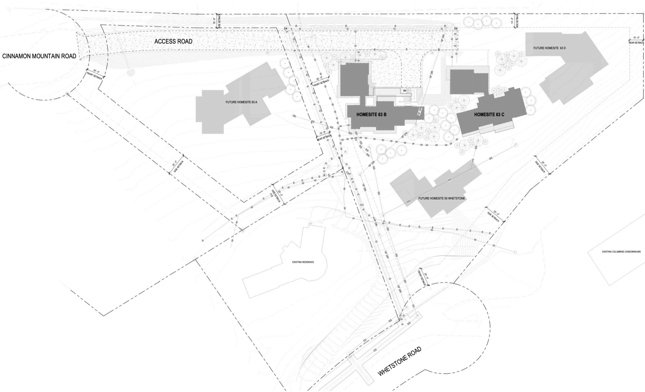
CINNAMON OVERALL SITE PLAN - 1:20 SCALE
