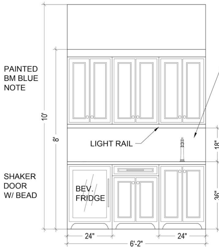
BUTLER CABINETRY DETAIL
