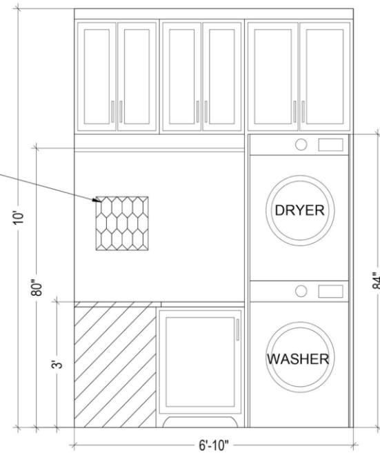
LAUNDRY ROOM ELEVATION
