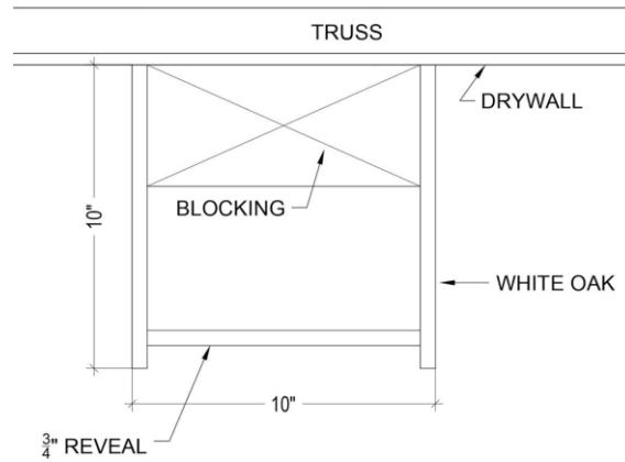
MASTER BEDROOM BEAM DETAIL SECTION
