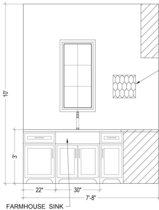
LAUNDRY ROOM ELEVATION
