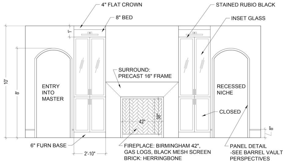
LIVING ROOM ELEVATION
