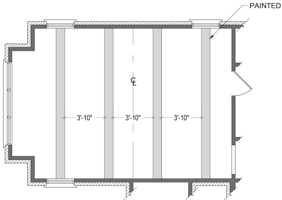
MASTER BEDROOM REFLECTED CEILING PLAN
