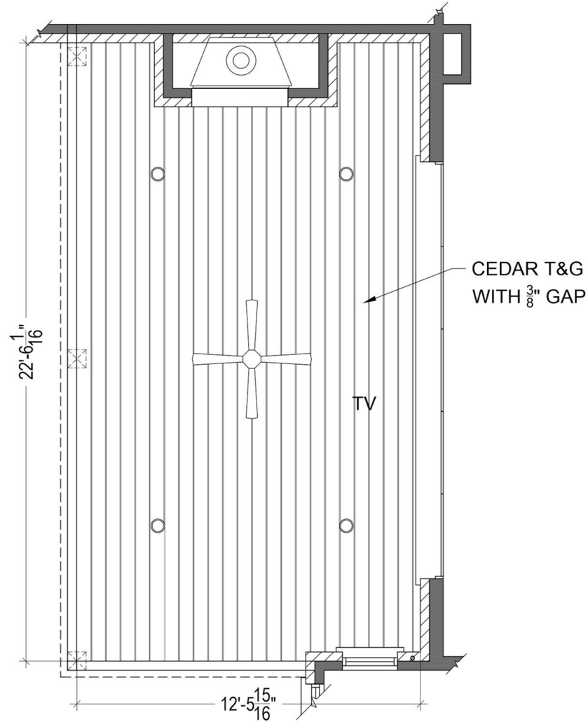
EXTERIOR PORCH RCP
