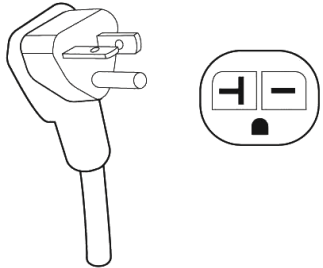
240volt / 20 amp NEMA 6-20 Plug
