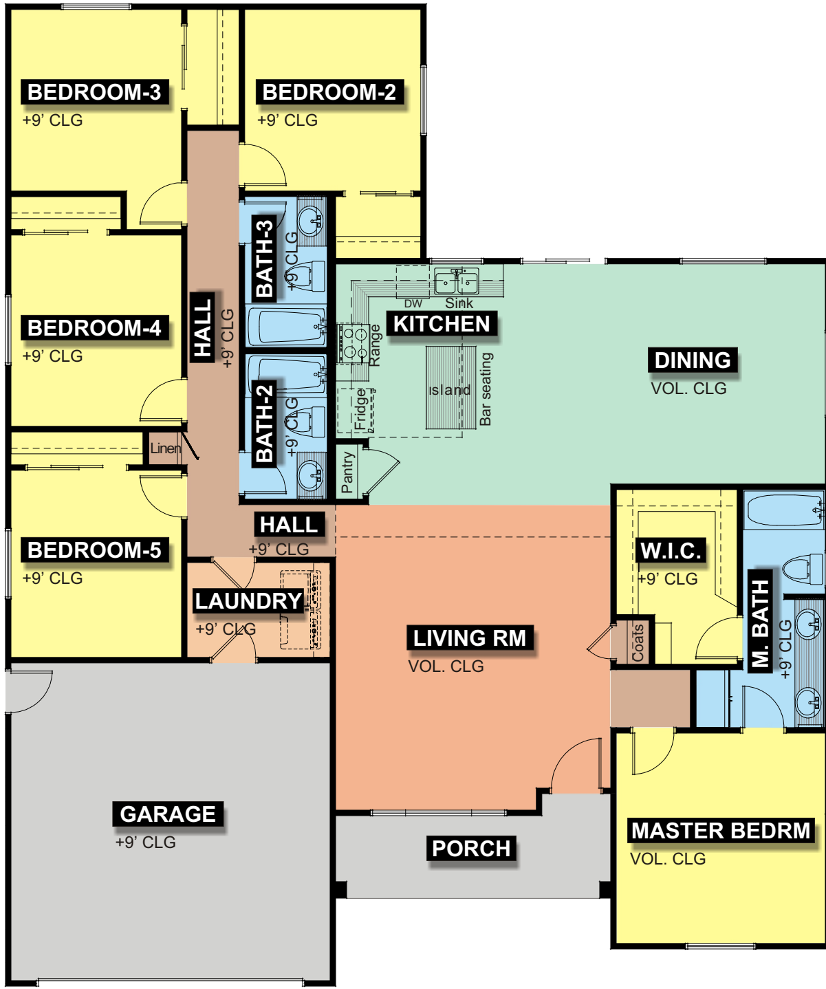
FLOOR PLAN 5 Bedroom - 3 Bath
