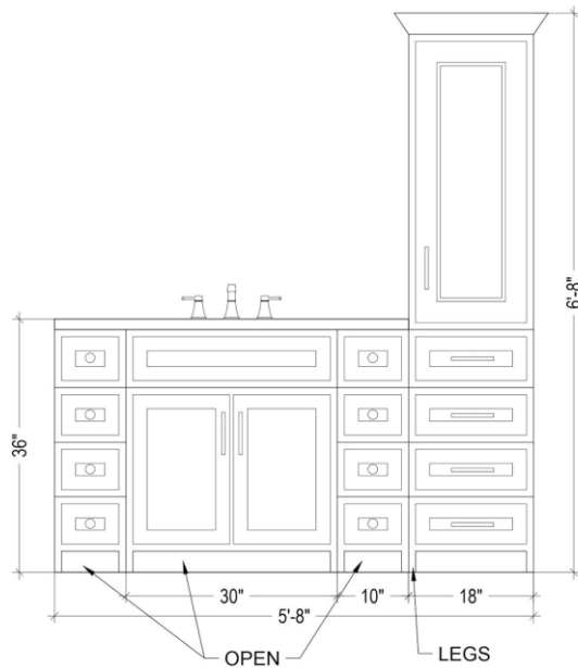
BATH 4 CABINETRY DETAILS
