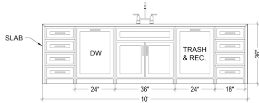
KITCHEN ISLAND CABINETS DETAILS
