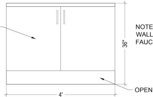
GUEST BATH CABINETS DETAILS
