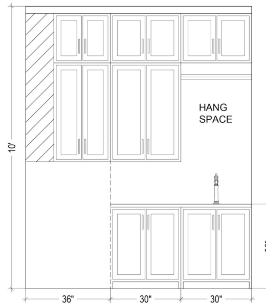
LAUNDRY - ELEVATION B
