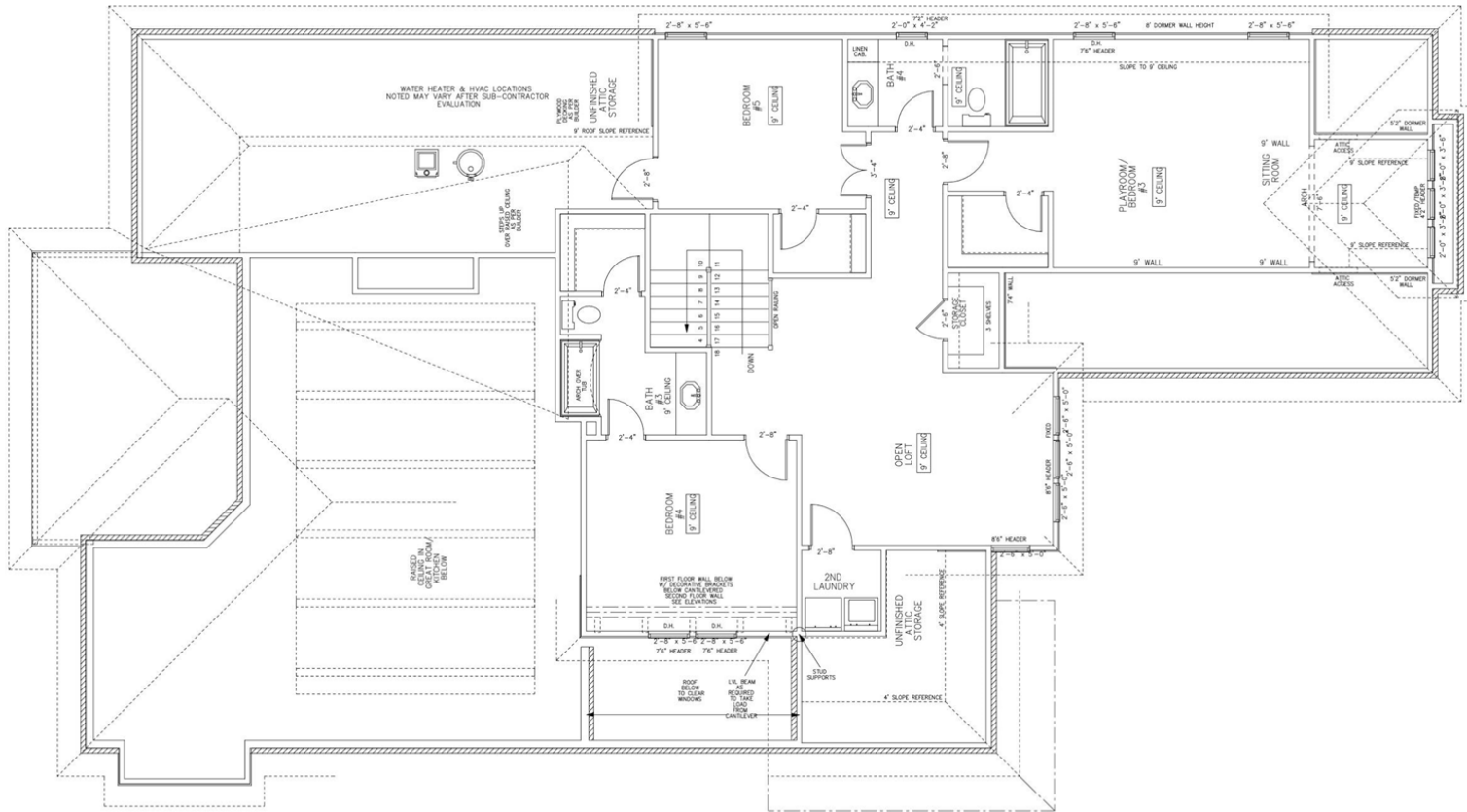
SECOND FLOOR DETAIL CONSTRUCTION SHEET SCALE: 1/4" = 1'-0"
