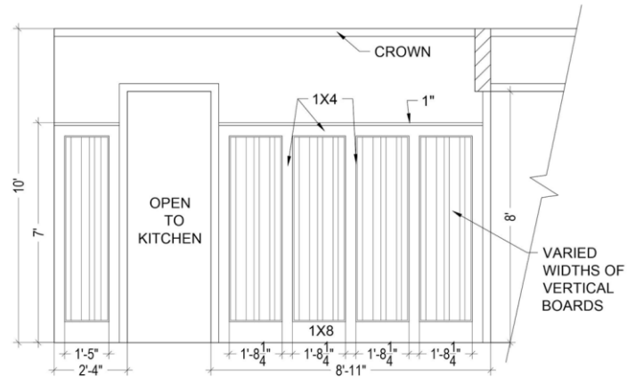
F DINING ROOM ELEVATION SCALE: 3/8" = 1'-0"
