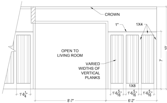
A SECOND FOYER ELEVATION SCALE: 3/8" = 1'-0"
