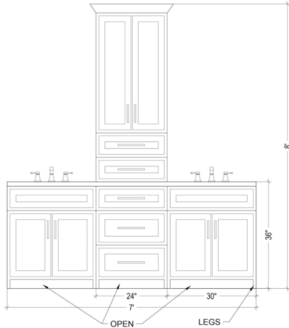
MASTER BATH CABINETS
