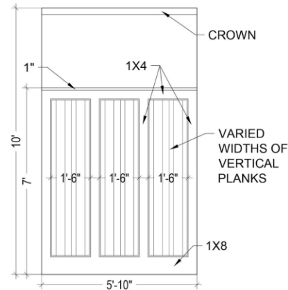
D SECOND FOYER ELEVATION SCALE: 3/8" = 1'-0"
