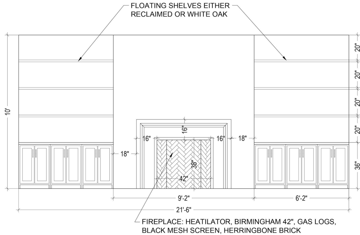
LIVING ROOM FIREPLACE ELEVATION
