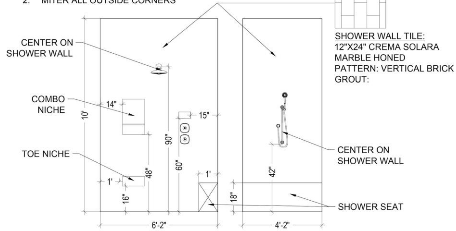
MASTER SHOWER ELEVATIONS
