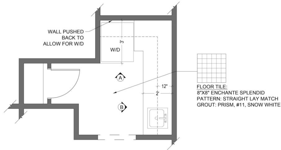
LAUNDRY 1ST FLOOR - FLOOR PLAN
