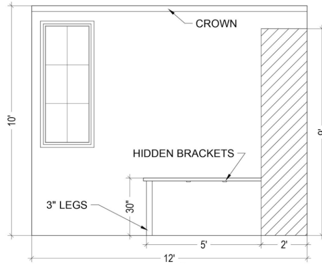
STUDY ELEVATION SCALE: 3/8" = 1'-0"
