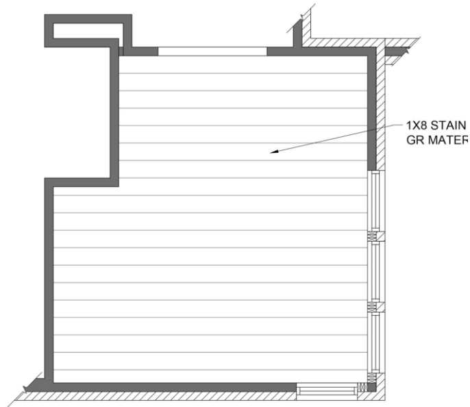
STUDY - RCP SCALE: 3/8" = 1'-0"
