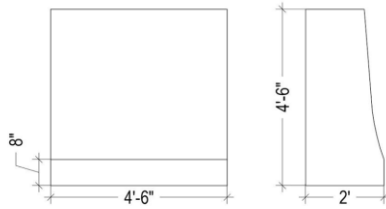
RANGE HOOD DETAILS
