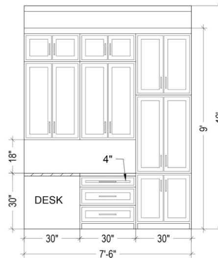
STUDY ELEVATION SCALE: 3/8" = 1'-0"
