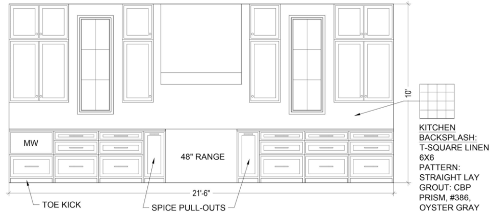
KITCHEN CABINETS DETAIL
