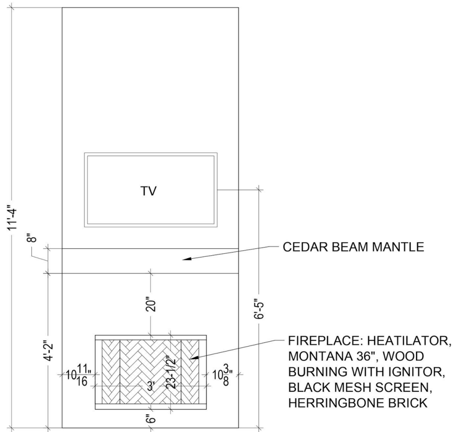
EXTERIOR FIREPLACE ELEVATION
