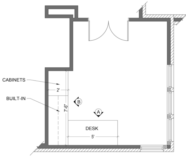
STUDY FLOOR PLAN SCALE: 3/8" = 1'-0"
