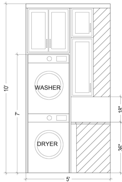
LAUNDRY - ELEVATION A
