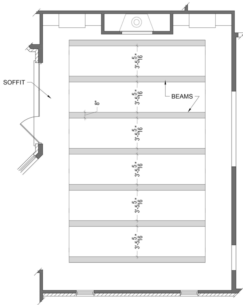
LIVING ROOM/ KITCHEN - RCP
