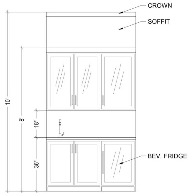
DINING ROOM WET BAR CABINETRY DETAILS
