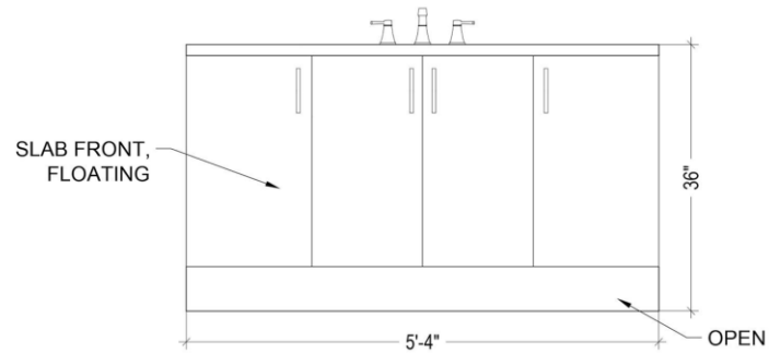
BATH 3 CABINETS DETAILS
