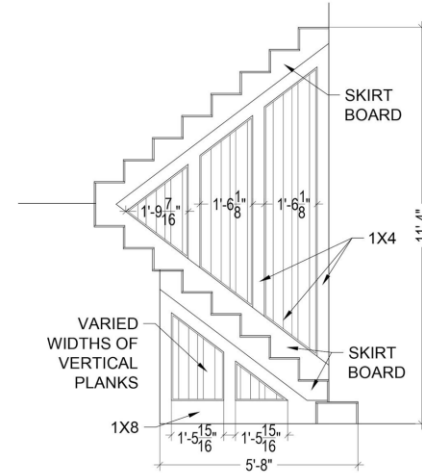
C SECOND FOYER ELEVATION SCALE: 3/8" = 1'-0"
