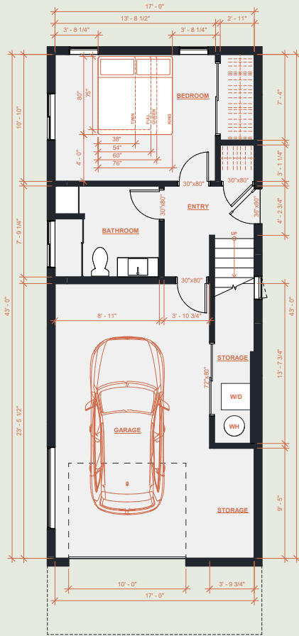
FLOOR PLAN - GROUND
