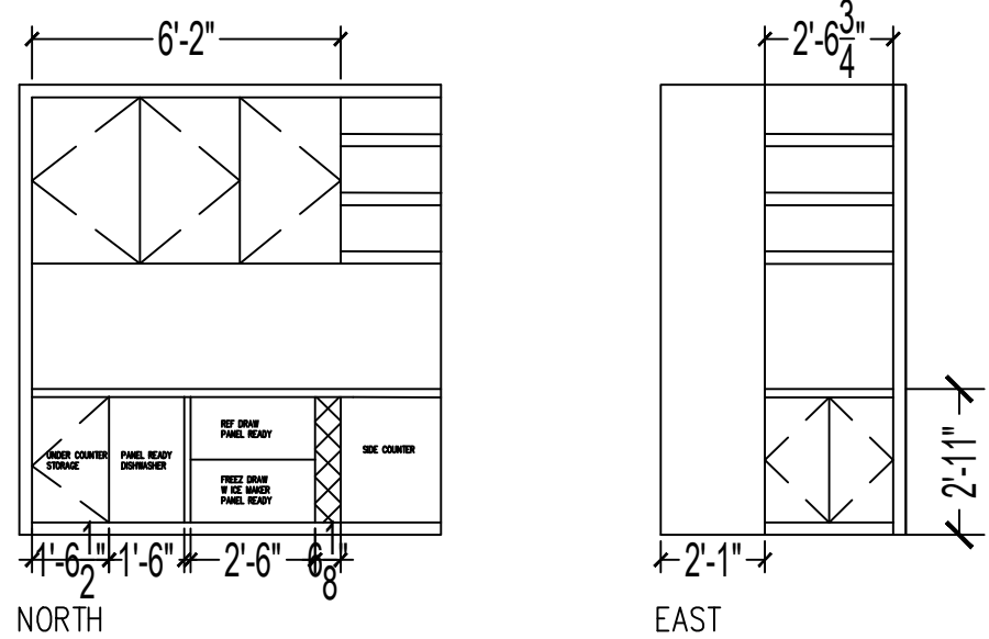
KITCHENETTE ELEVATION
